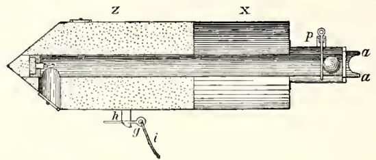
FIG. 2. CUSHING'S TORPEDO—SECTIONAL VIEW.
